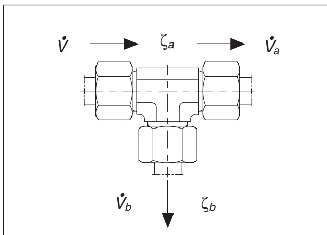
Pipe branching
