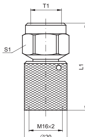
Gauge-Direct-Connector: MAVMD...MA3
